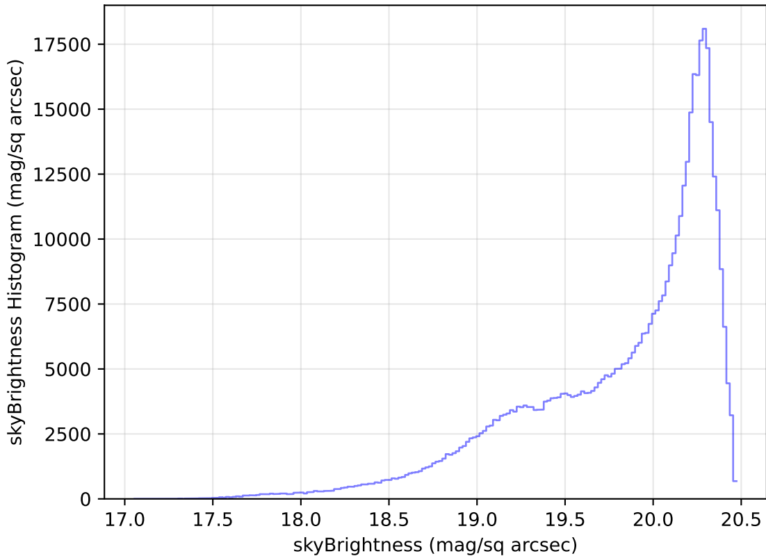
weather_cloudso16v3.4_10yrs All sky i band: skyBrightness Histogram
