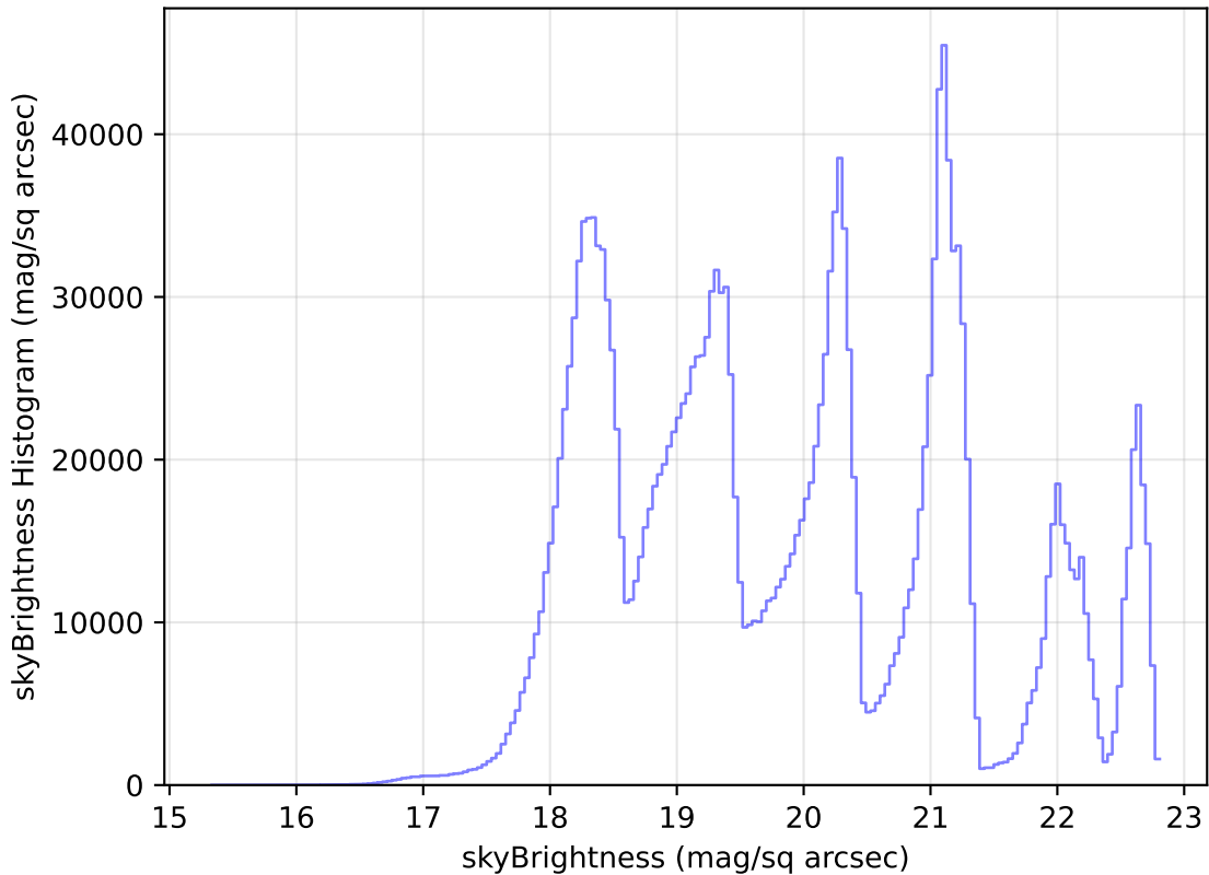
weather_cloudso16v3.4_10yrs All sky all bands: skyBrightness Histogram
