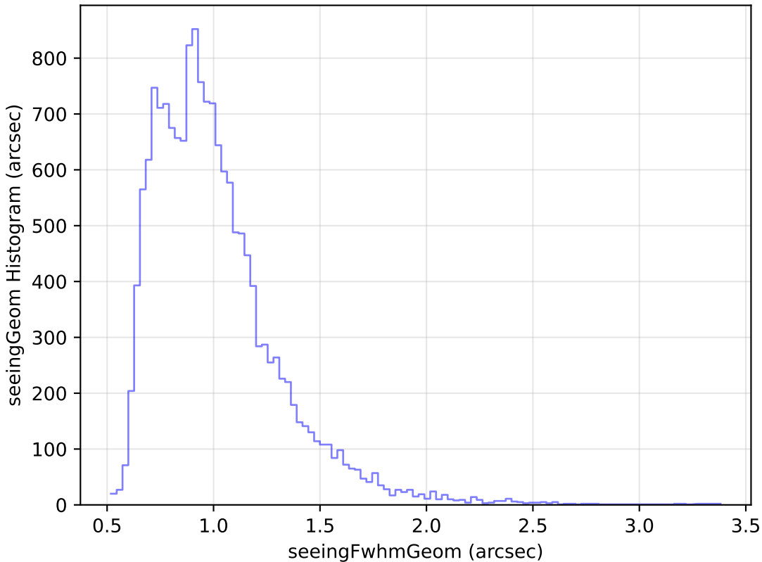
weather_cloudso16v3.4_10yrs Yr 1 u band: seeingGeom Histogram
