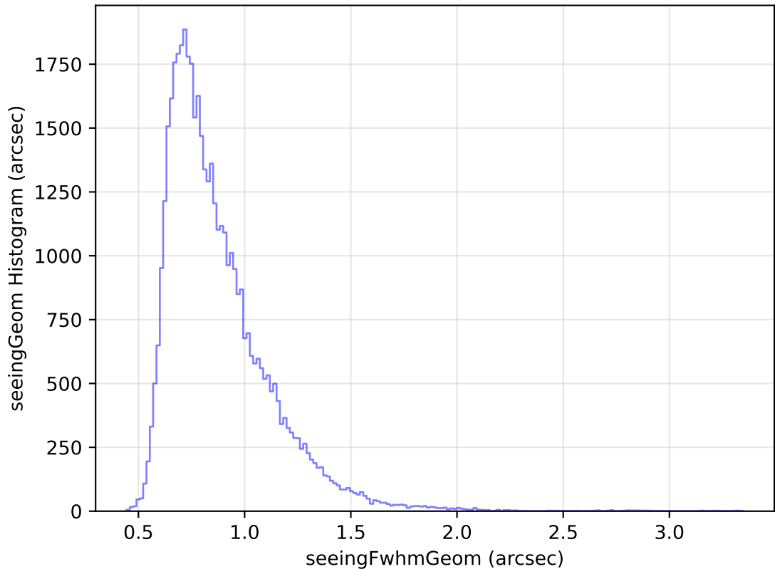
weather_cloudso16v3.4_10yrs Yr 1 r band: seeingGeom Histogram
