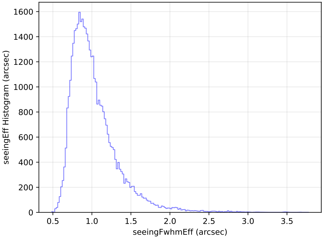
weather_cloudso16v3.4_10yrs Yr 1 z band: seeingEff Histogram
