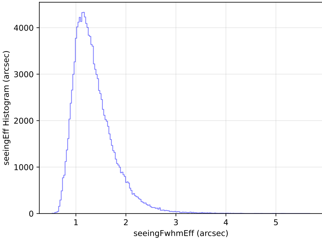
weather_cloudso16v3.4_10yrs WFD u band: seeingEff Histogram
