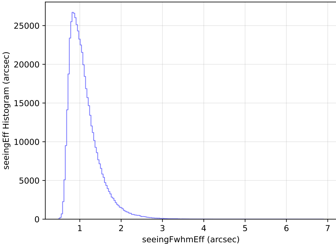
weather_cloudso16v3.4_10yrs WFD i band: seeingEff Histogram
