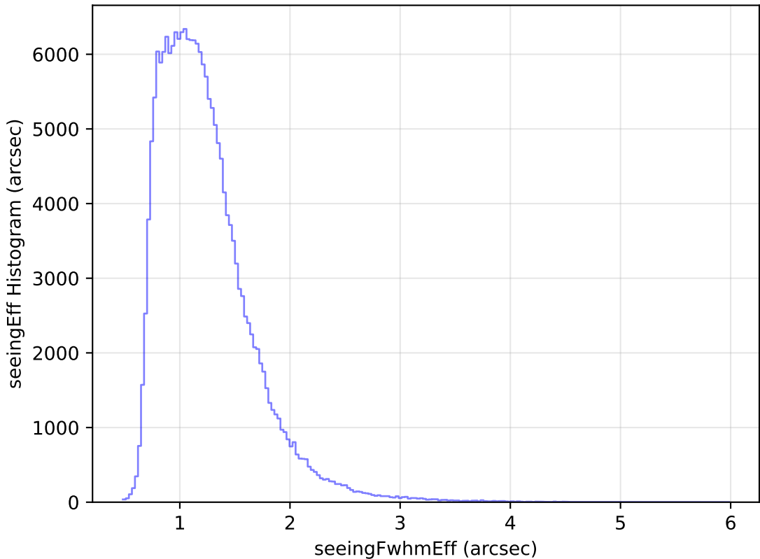
weather_cloudso16v3.4_10yrs WFD g band: seeingEff Histogram
