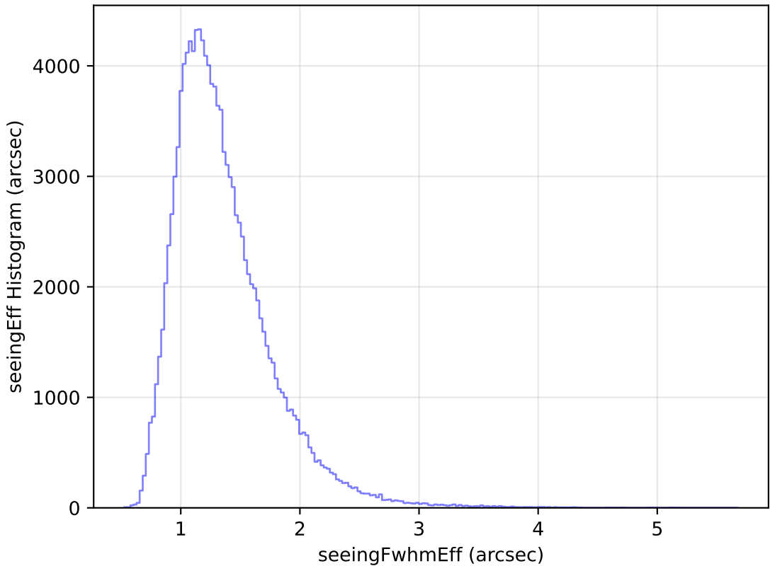
weather_cloudso16v3.4_10yrs All sky u band: seeingEff Histogram
