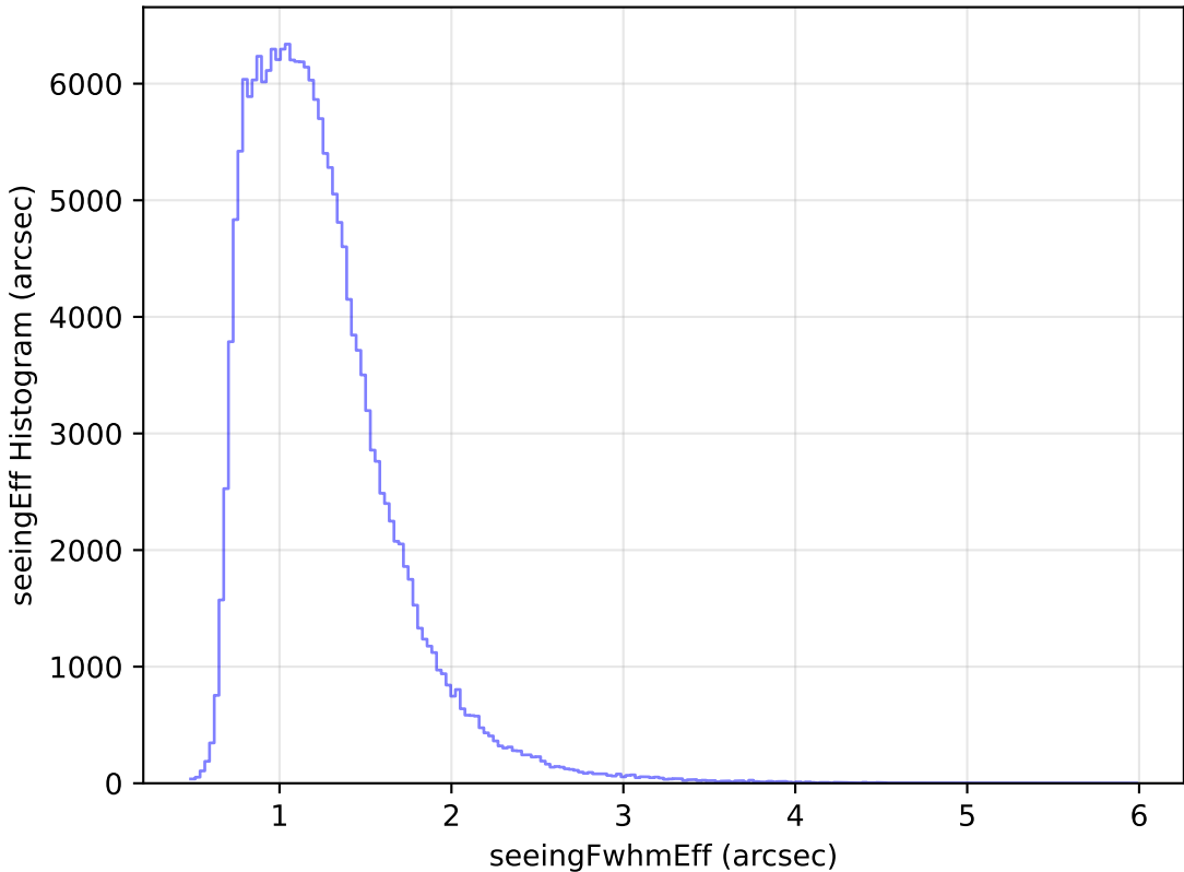
weather_cloudso16v3.4_10yrs All sky g band: seeingEff Histogram
