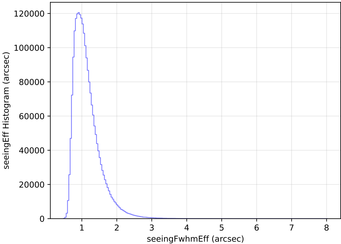
weather_cloudso16v3.4_10yrs All sky all bands: seeingEff Histogram
