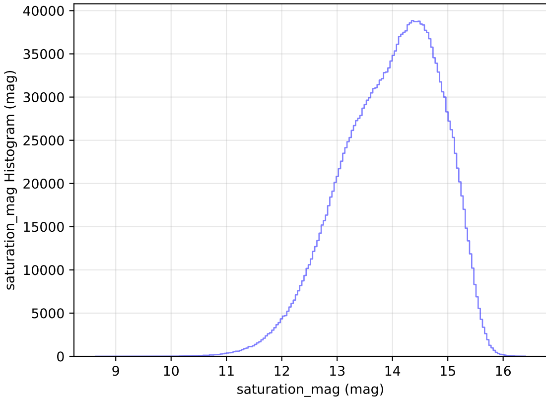
weather_cloudso16v3.4_10yrs All sky all bands: saturation_mag Histogram
