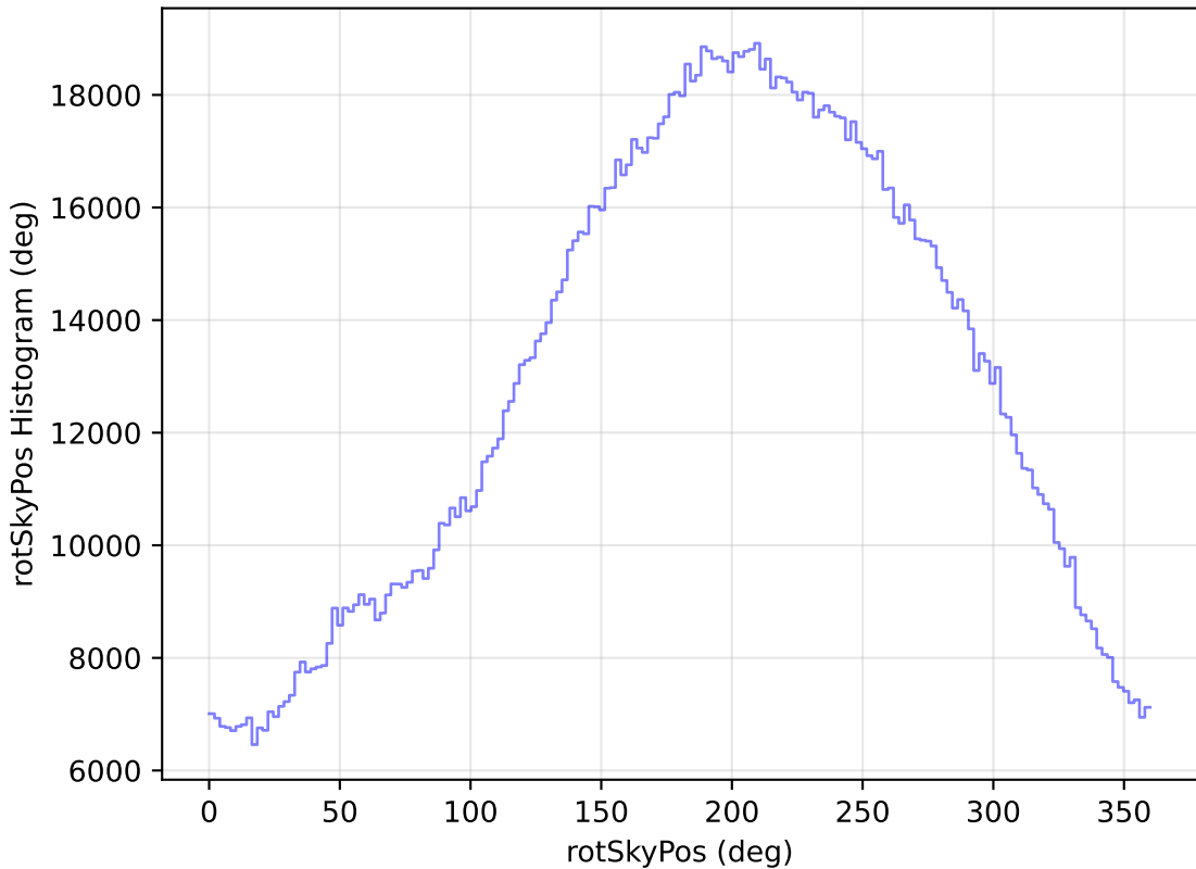
weather_cloudso16v3.4_10yrs All sky all bands: rotSkyPos Histogram
