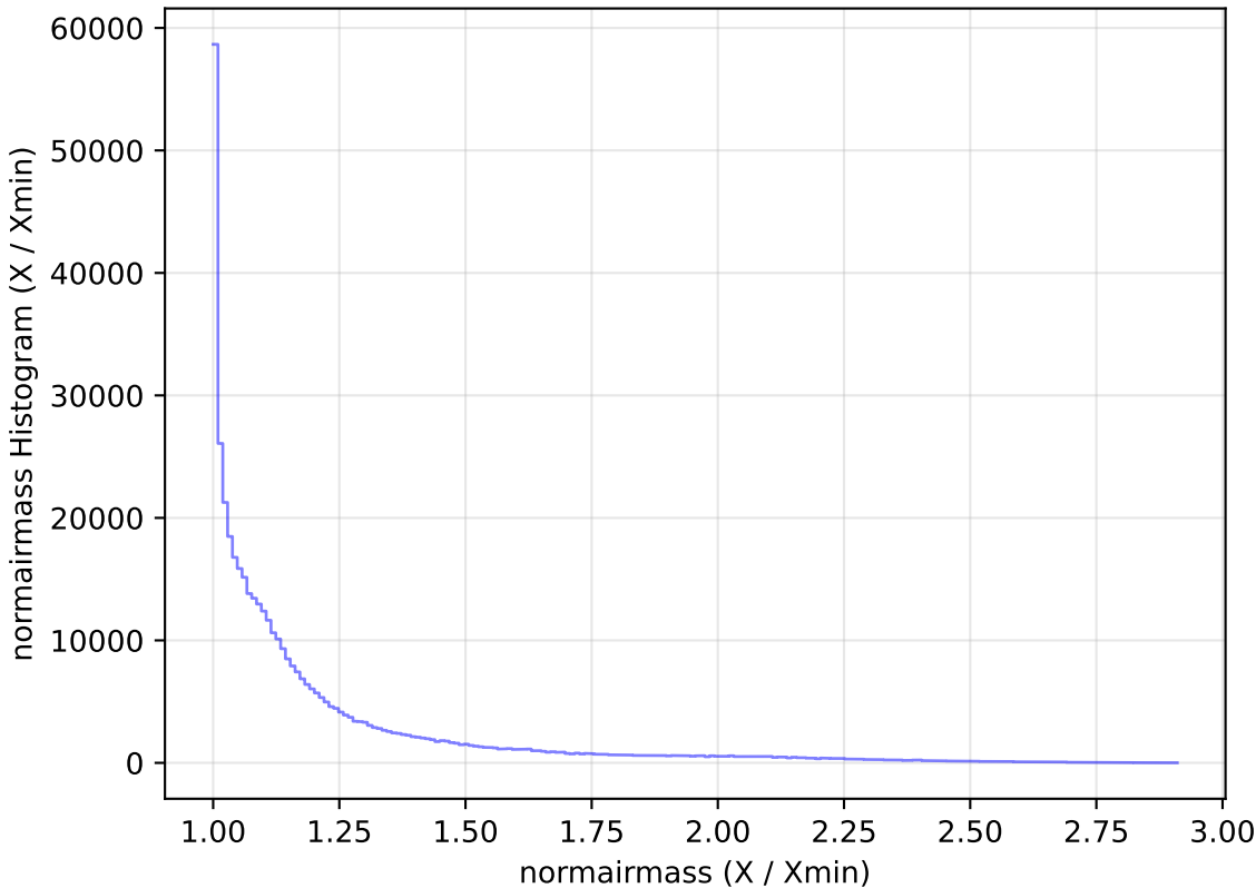
weather_cloudso16v3.4_10yrs WFD z band: normairmass Histogram
