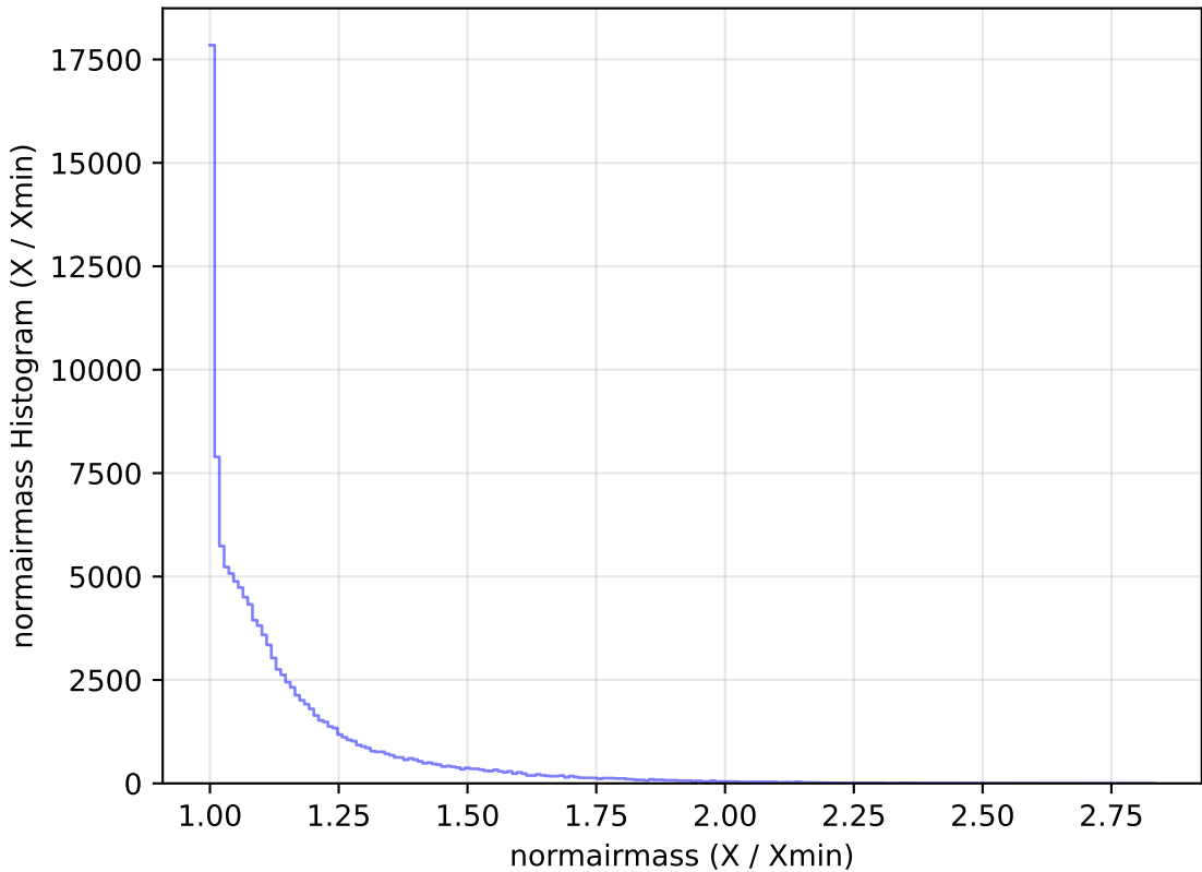
weather_cloudso16v3.4_10yrs WFD u band: normairmass Histogram
