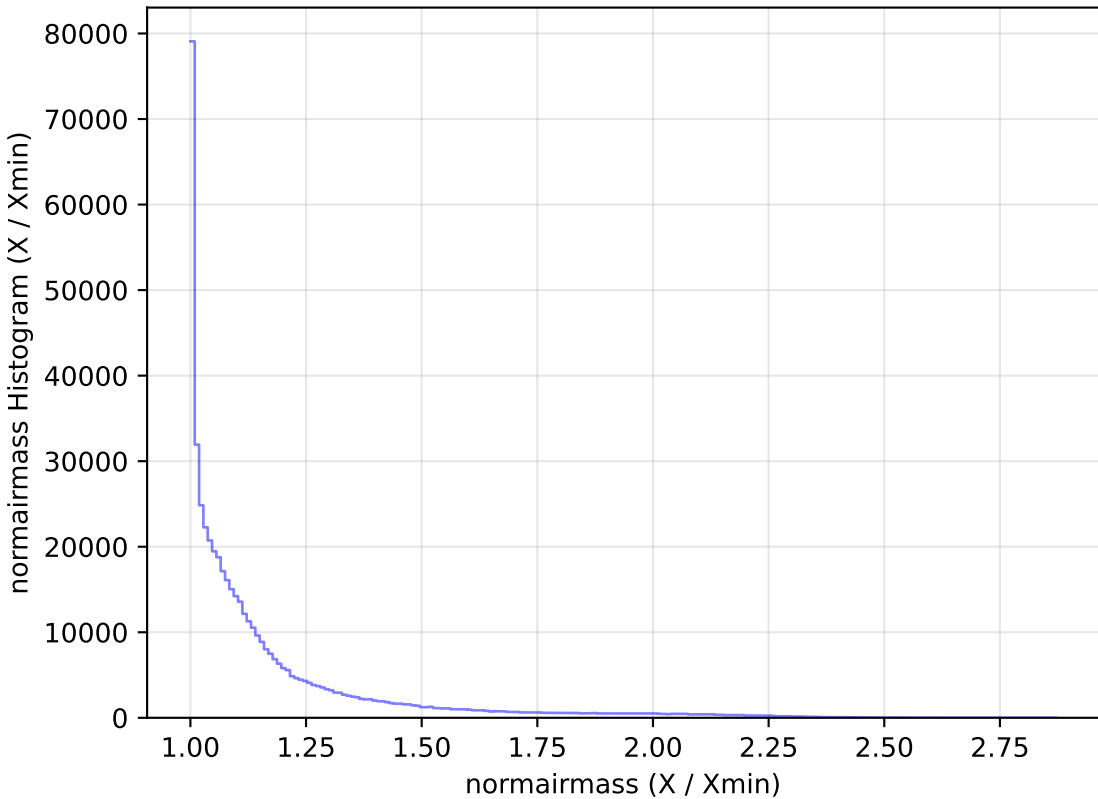
weather_cloudso16v3.4_10yrs WFD r band: normairmass Histogram
