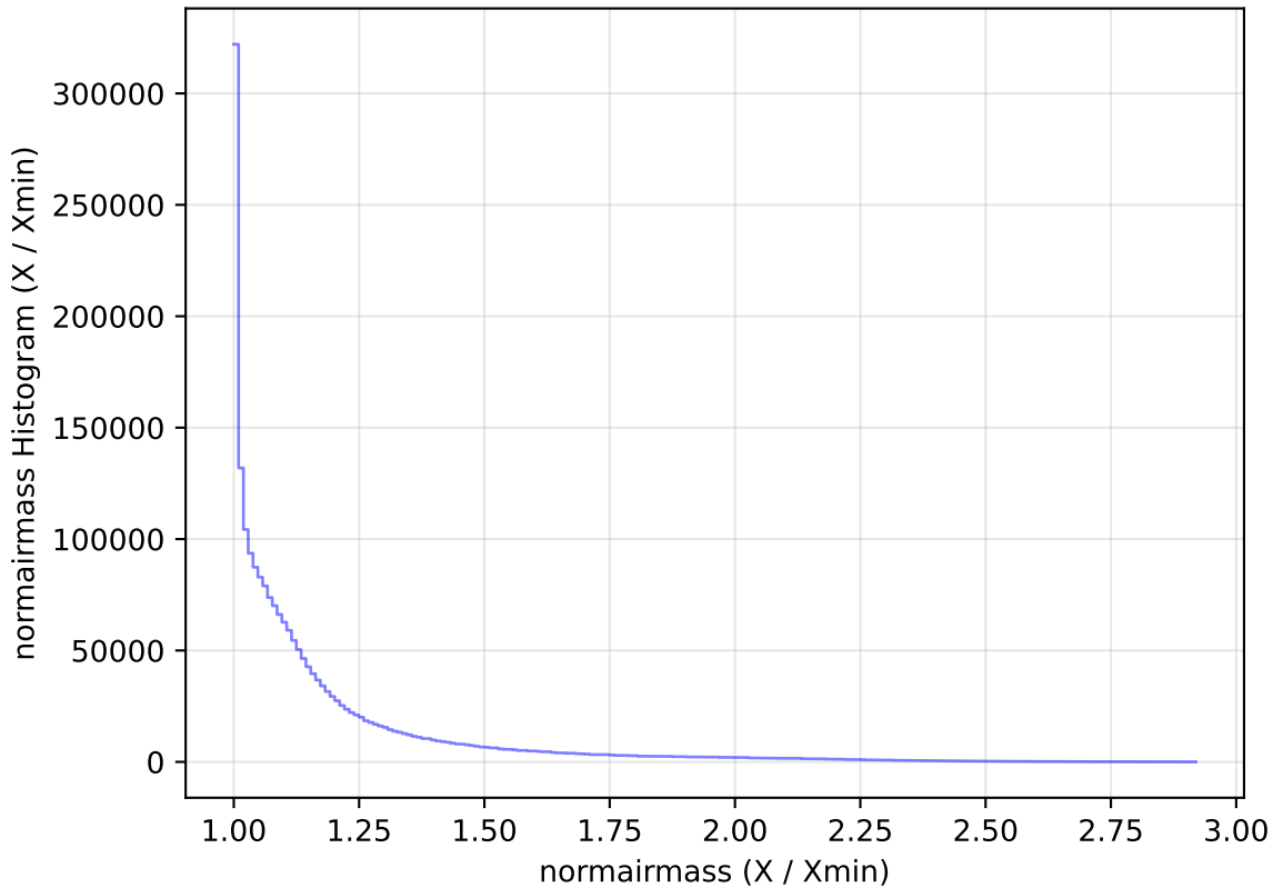
weather_cloudso16v3.4_10yrs WFD all bands: normairmass Histogram
