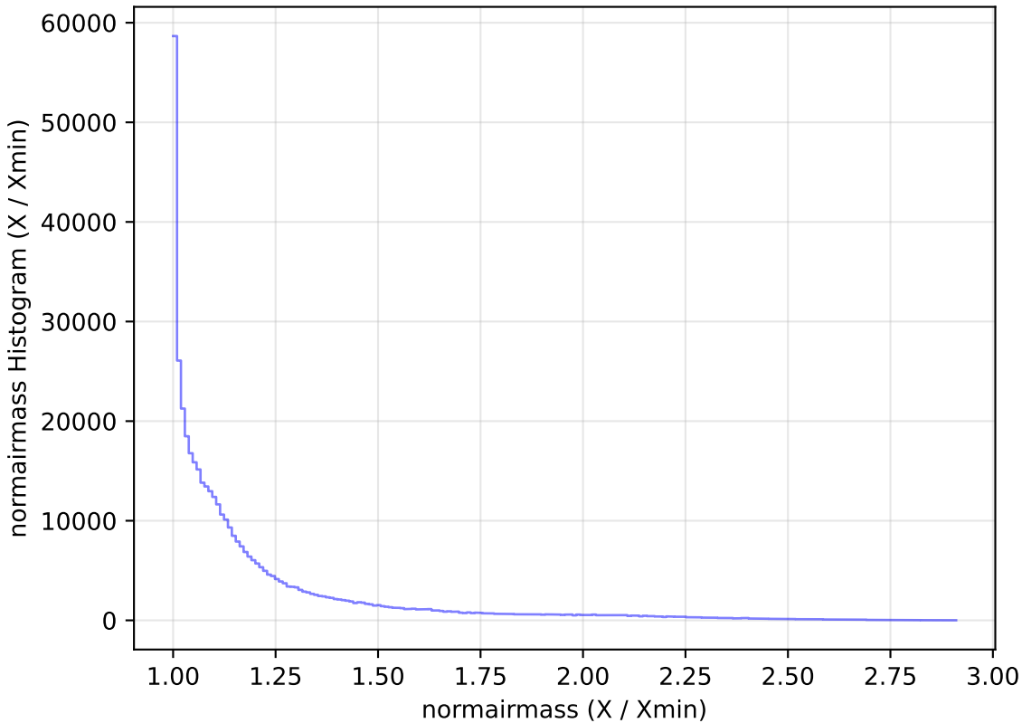
weather_cloudso16v3.4_10yrs All sky z band: normairmass Histogram
