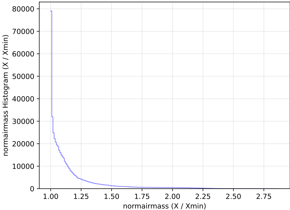
weather_cloudso16v3.4_10yrs All sky r band: normairmass Histogram
