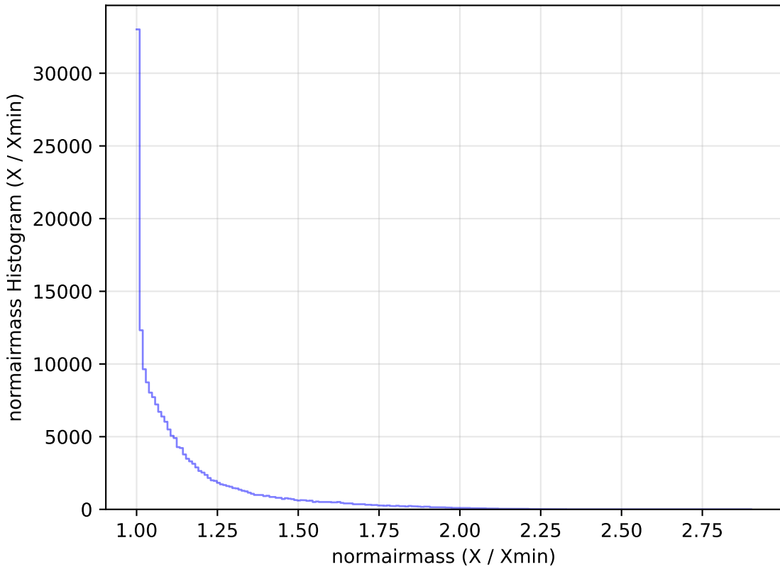
weather_cloudso16v3.4_10yrs All sky g band: normairmass Histogram
