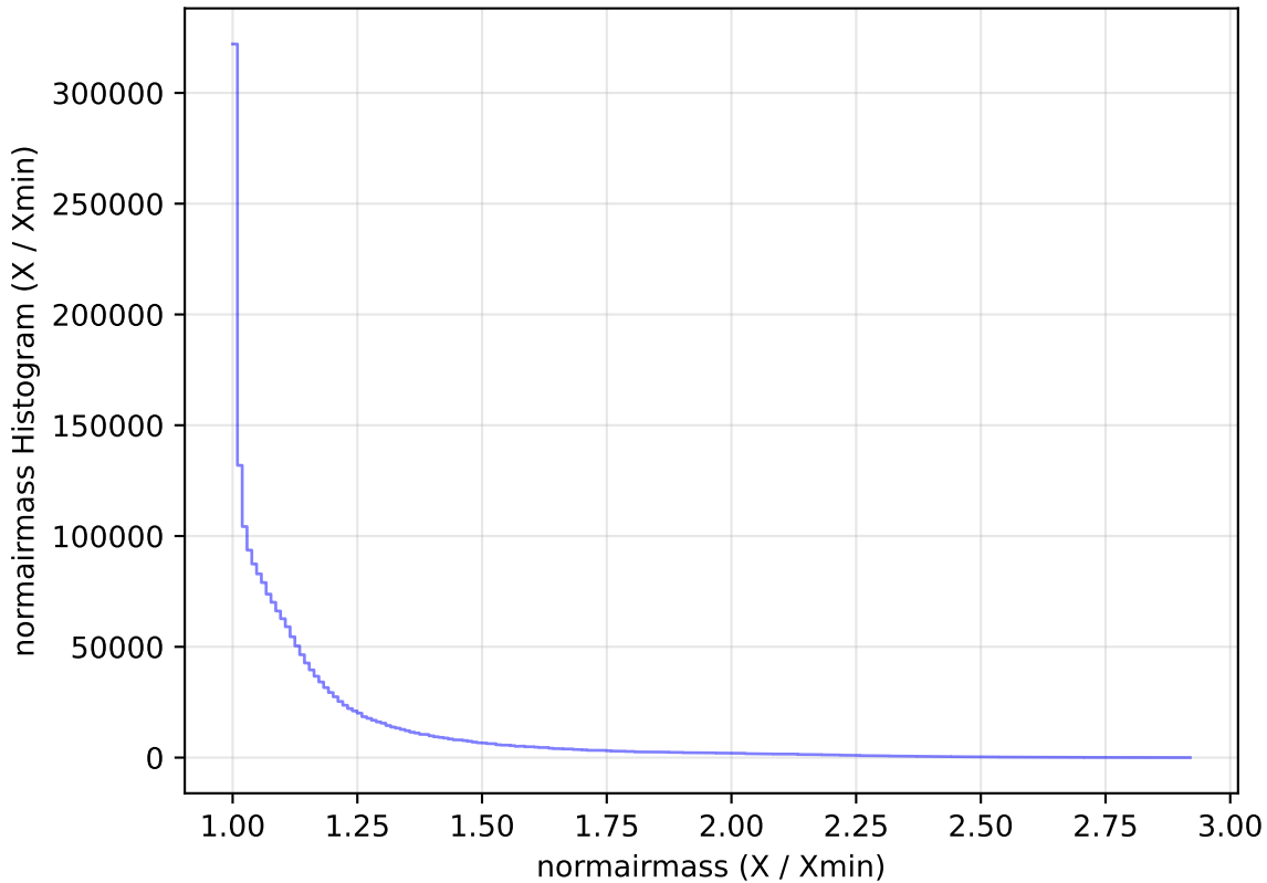
weather_cloudso16v3.4_10yrs All sky all bands: normairmass Histogram
