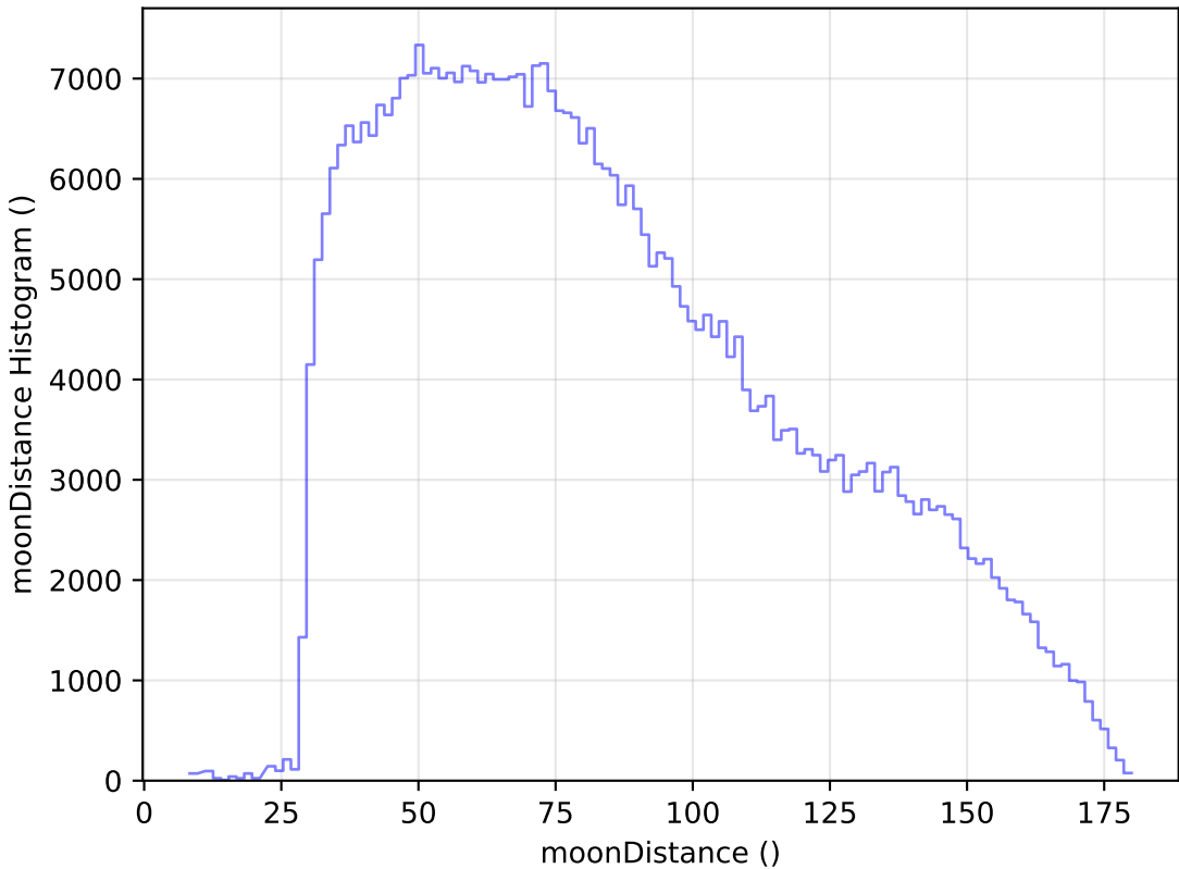
weather_cloudso16v3.4_10yrs WFD z band: moonDistance Histogram
