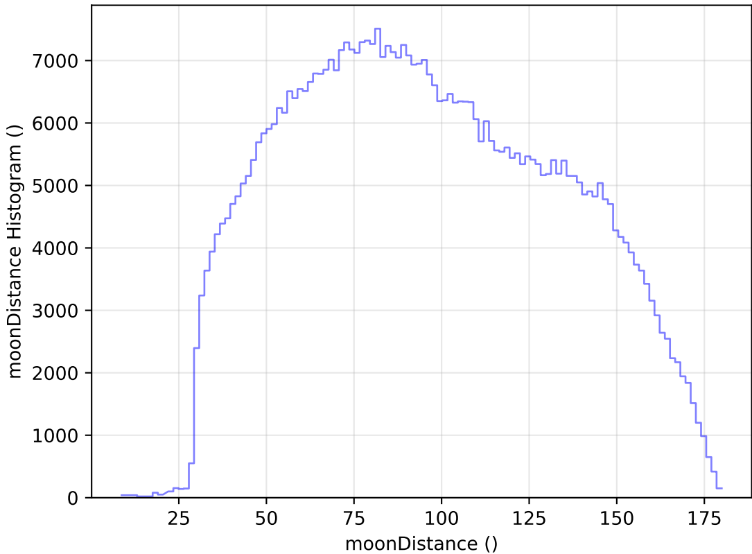
weather_cloudso16v3.4_10yrs WFD i band: moonDistance Histogram
