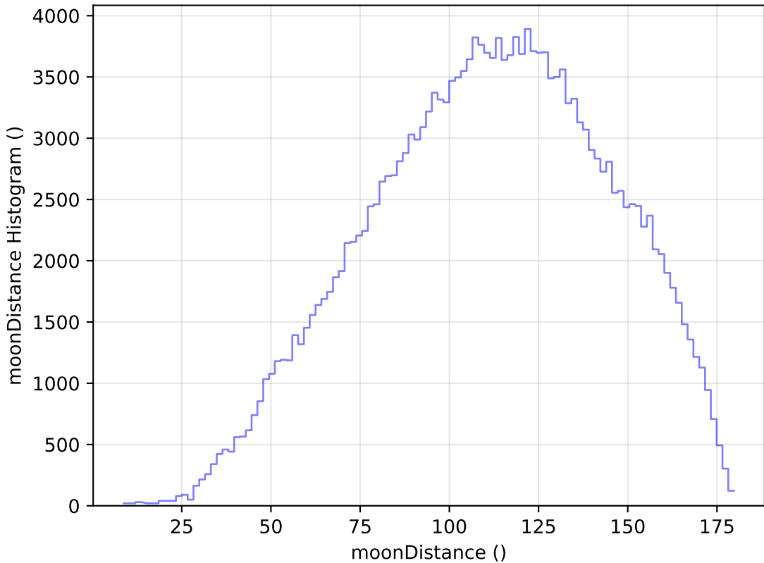
weather_cloudso16v3.4_10yrs WFD g band: moonDistance Histogram
