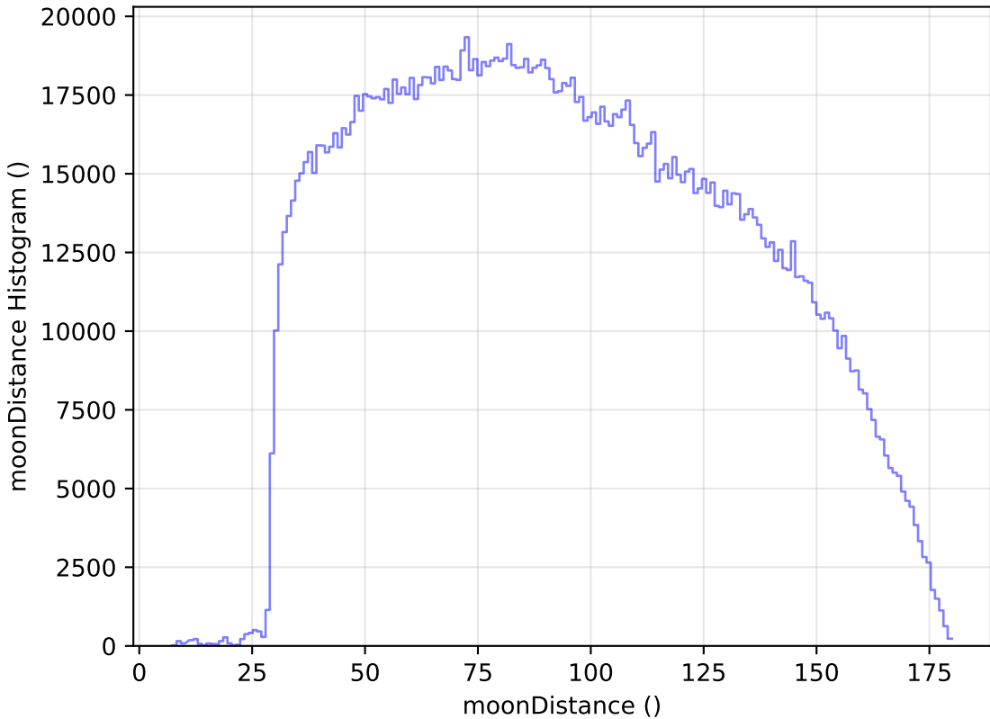
weather_cloudso16v3.4_10yrs WFD all bands: moonDistance Histogram
