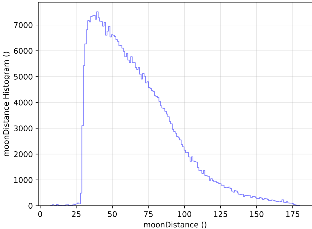
weather_cloudso16v3.4_10yrs All sky y band: moonDistance Histogram
