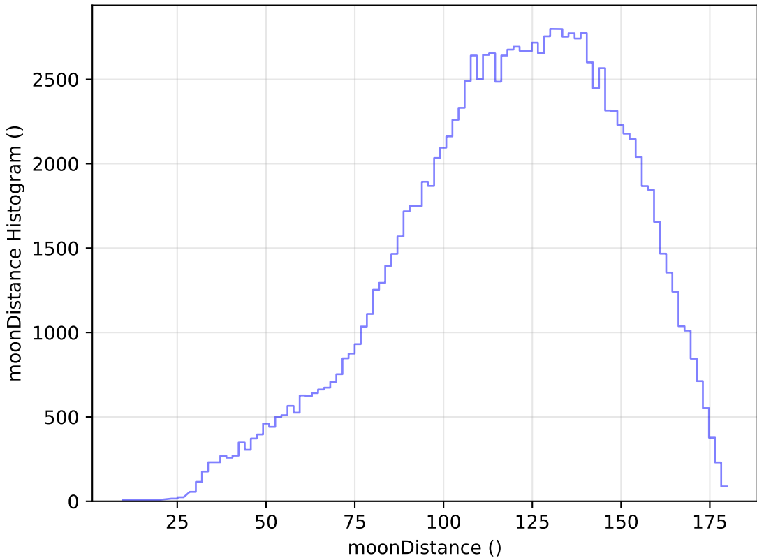
weather_cloudso16v3.4_10yrs All sky u band: moonDistance Histogram
