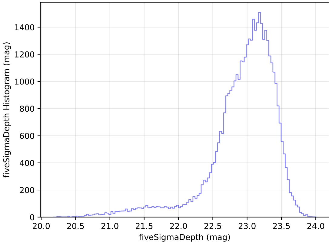
weather_cloudso16v3.4_10yrs Yr 1 z band: fiveSigmaDepth Histogram
