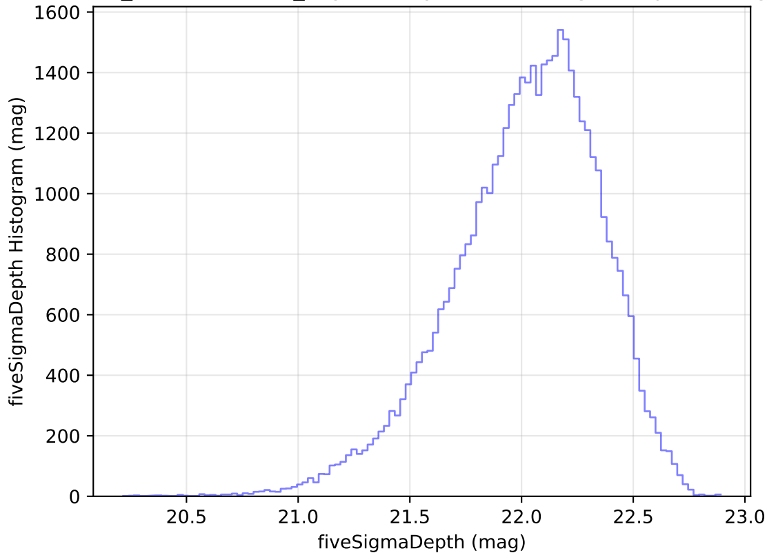
weather_cloudso16v3.4_10yrs Yr 1 y band: fiveSigmaDepth Histogram
