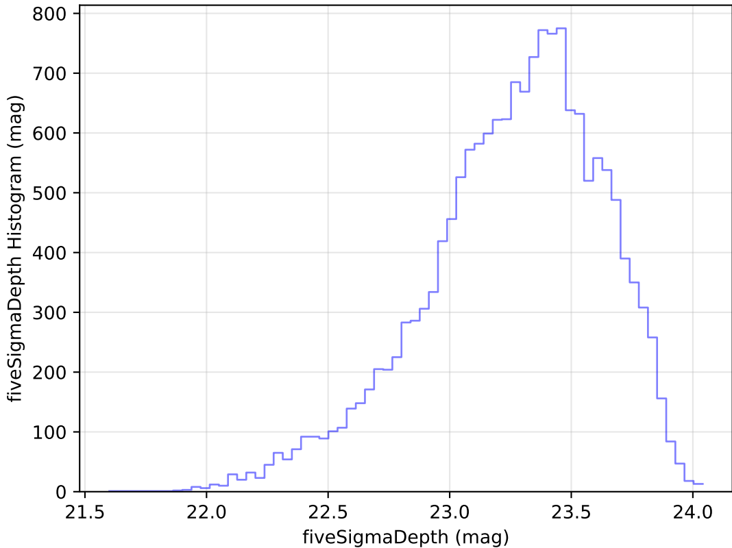
weather_cloudso16v3.4_10yrs Yr 1 u band: fiveSigmaDepth Histogram
