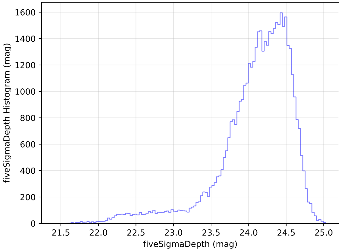
weather_cloudso16v3.4_10yrs Yr 1 r band: fiveSigmaDepth Histogram
