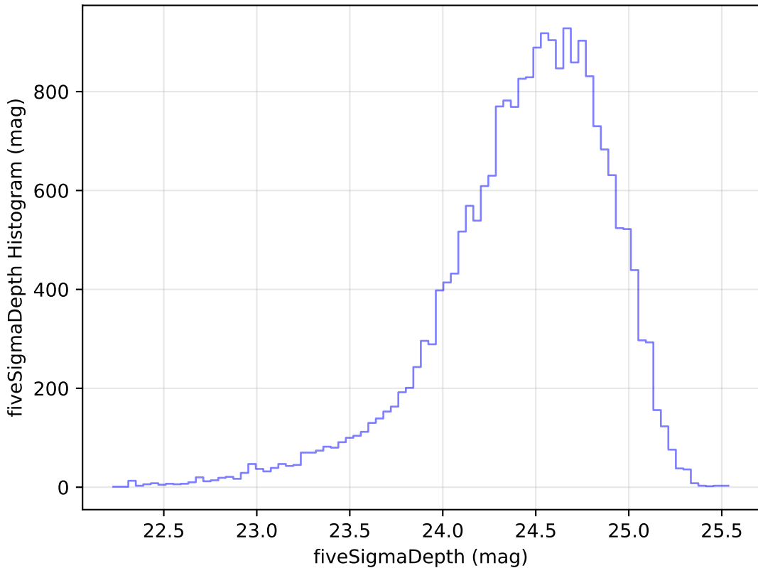
weather_cloudso16v3.4_10yrs Yr 1 g band: fiveSigmaDepth Histogram
