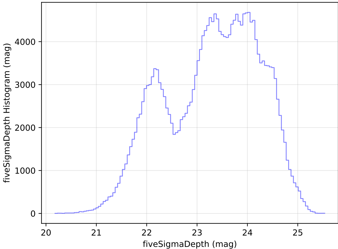
weather_cloudso16v3.4_10yrs Yr 1 all bands: fiveSigmaDepth Histogram
