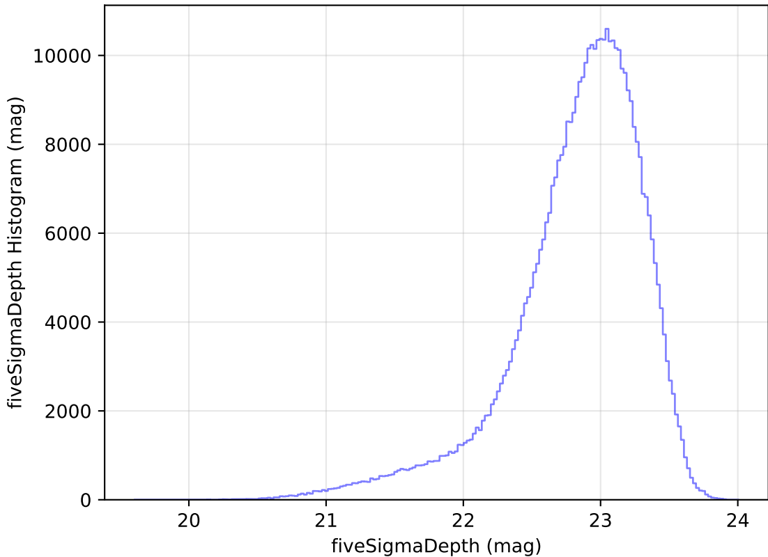
weather_cloudso16v3.4_10yrs WFD z band: fiveSigmaDepth Histogram
