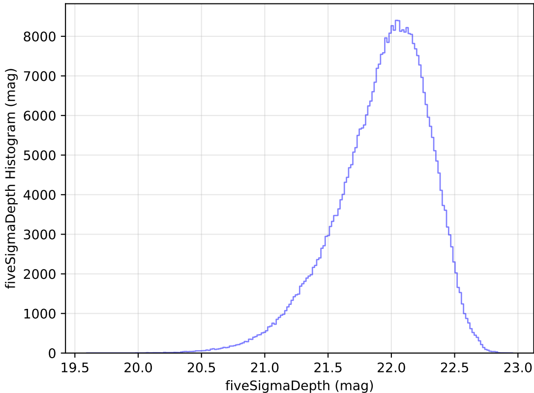
weather_cloudso16v3.4_10yrs WFD y band: fiveSigmaDepth Histogram
