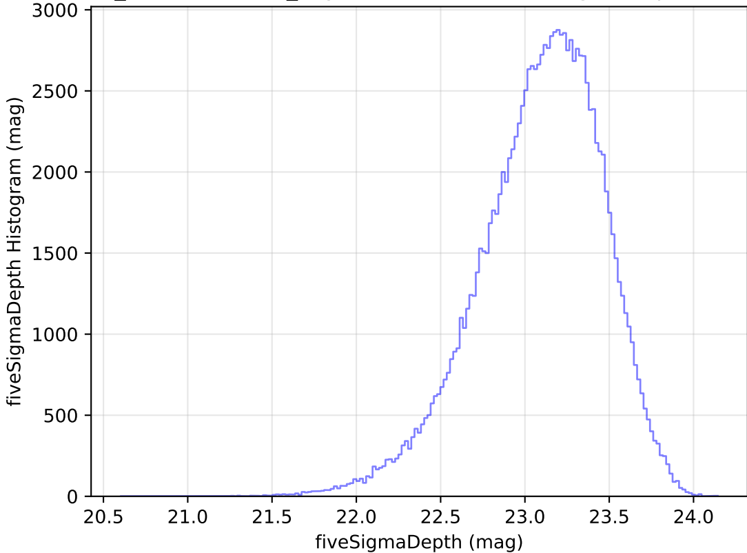
weather_cloudso16v3.4_10yrs WFD u band: fiveSigmaDepth Histogram
