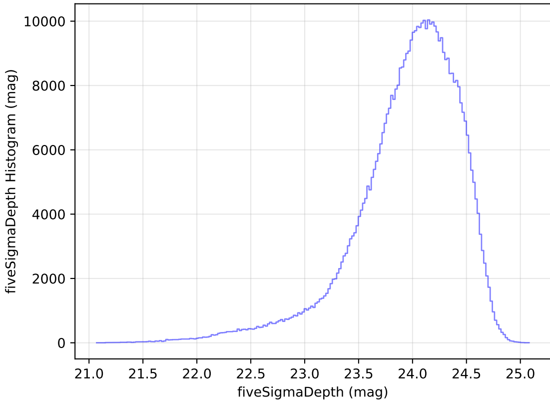
weather_cloudso16v3.4_10yrs WFD r band: fiveSigmaDepth Histogram
