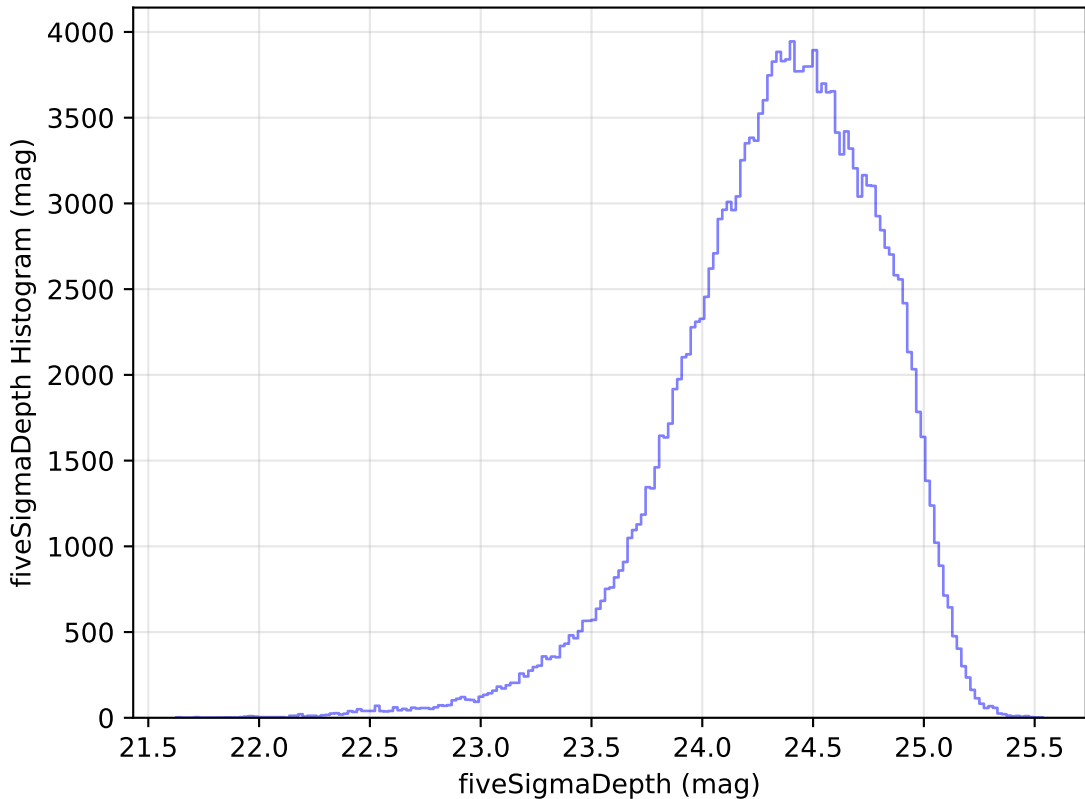
weather_cloudso16v3.4_10yrs WFD g band: fiveSigmaDepth Histogram
