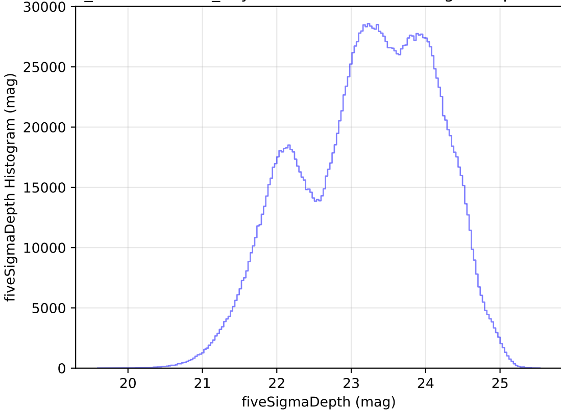
weather_cloudso16v3.4_10yrs WFD all bands: fiveSigmaDepth Histogram
