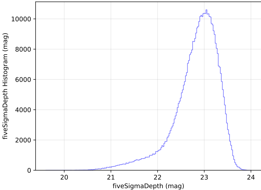
weather_cloudso16v3.4_10yrs All sky z band: fiveSigmaDepth Histogram
