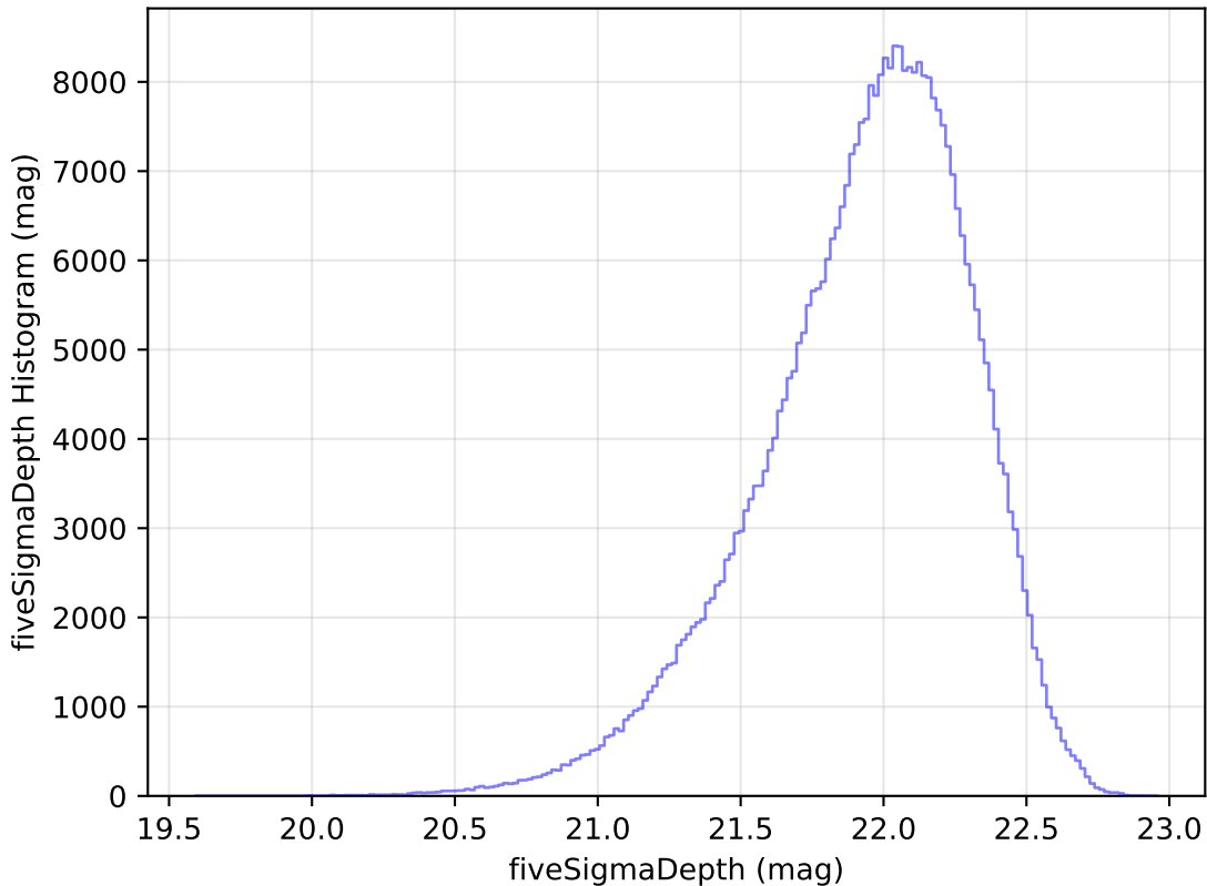
weather_cloudso16v3.4_10yrs All sky y band: fiveSigmaDepth Histogram
