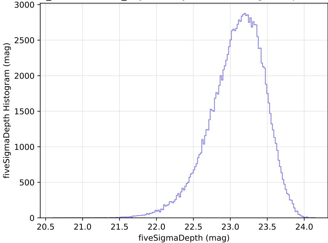
weather_cloudso16v3.4_10yrs All sky u band: fiveSigmaDepth Histogram
