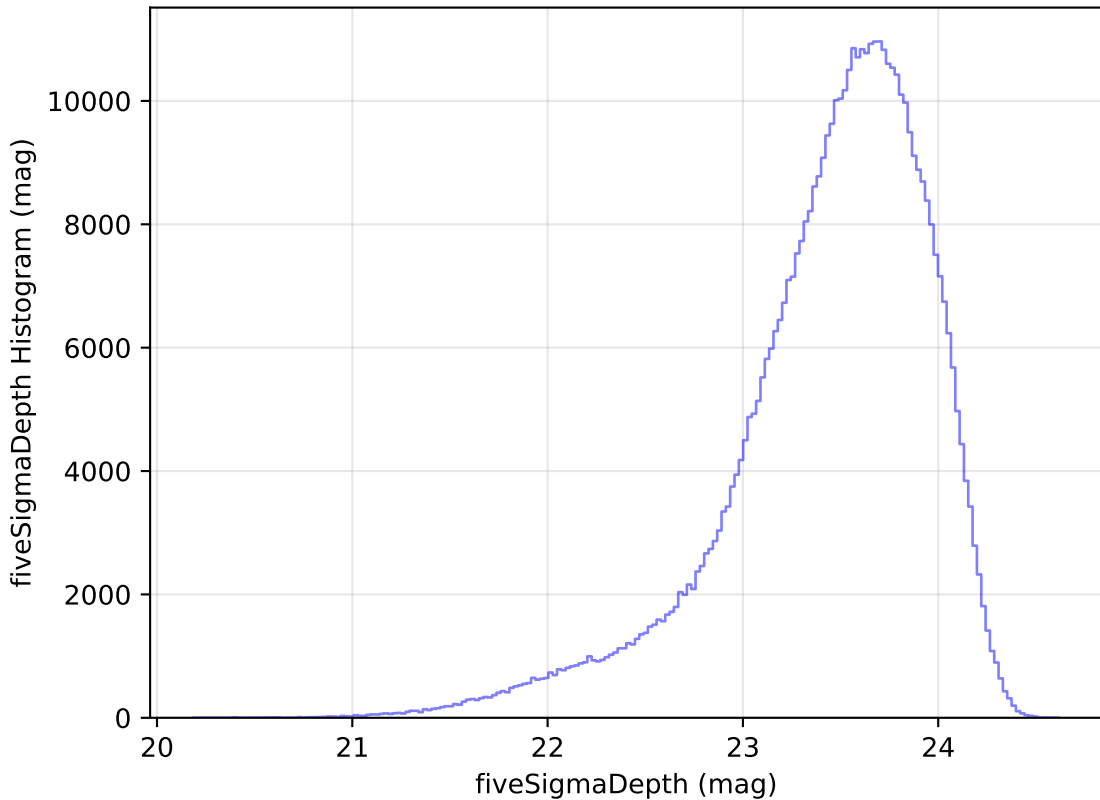
weather_cloudso16v3.4_10yrs All sky i band: fiveSigmaDepth Histogram
