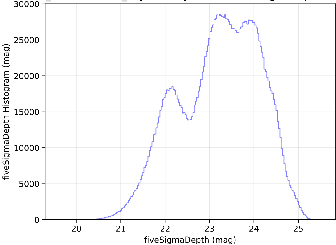
weather_cloudso16v3.4_10yrs All sky all bands: fiveSigmaDepth Histogram
