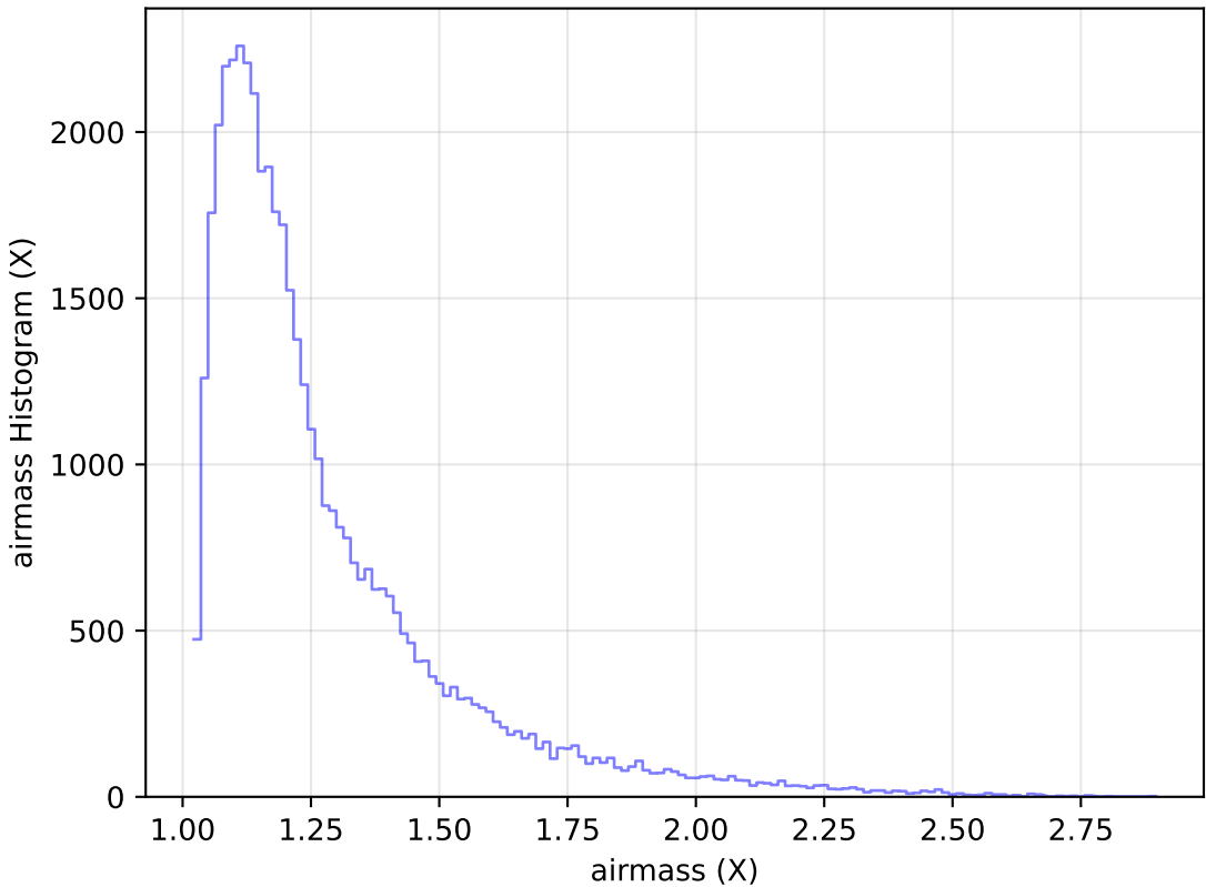
weather_cloudso16v3.4_10yrs Yr 1 y band: airmass Histogram
