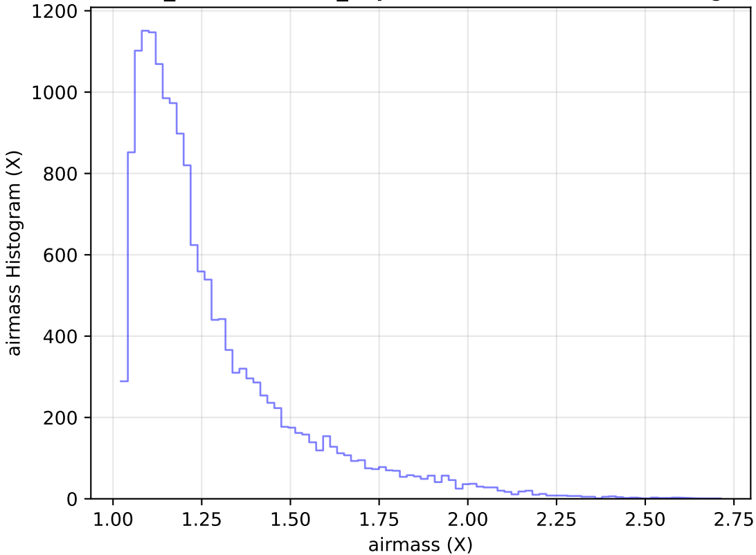
weather_cloudso16v3.4_10yrs Yr 1 u band: airmass Histogram
