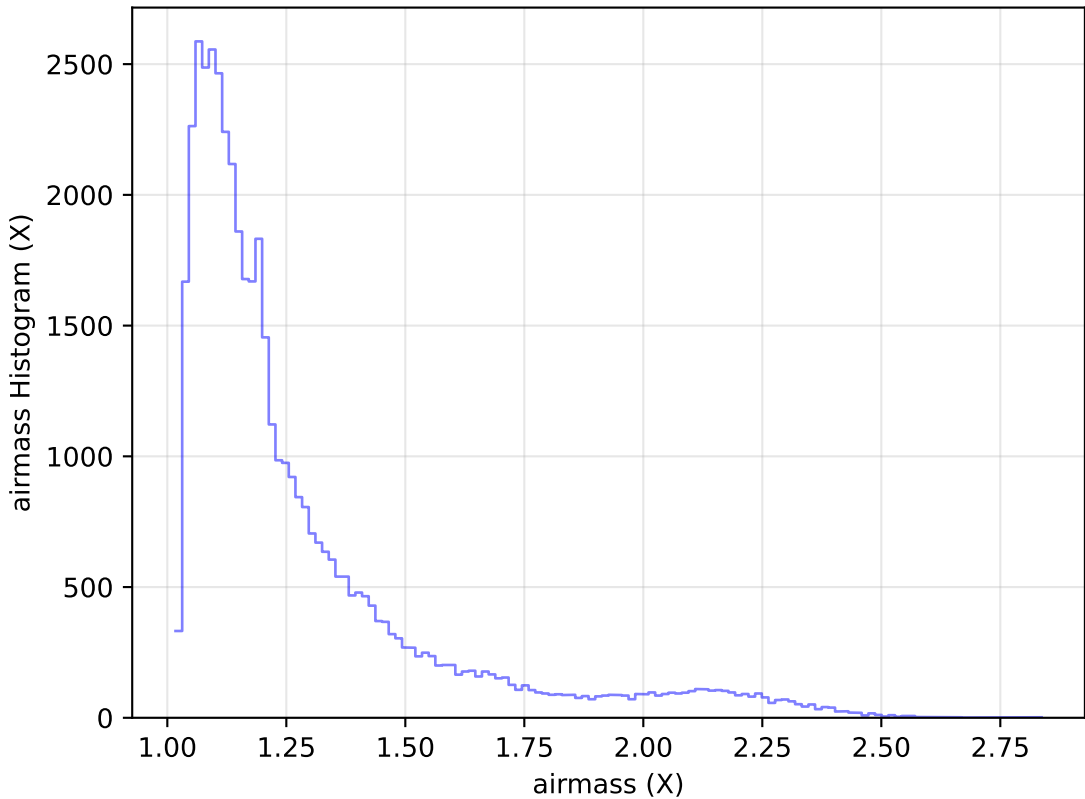
weather_cloudso16v3.4_10yrs Yr 1 r band: airmass Histogram
