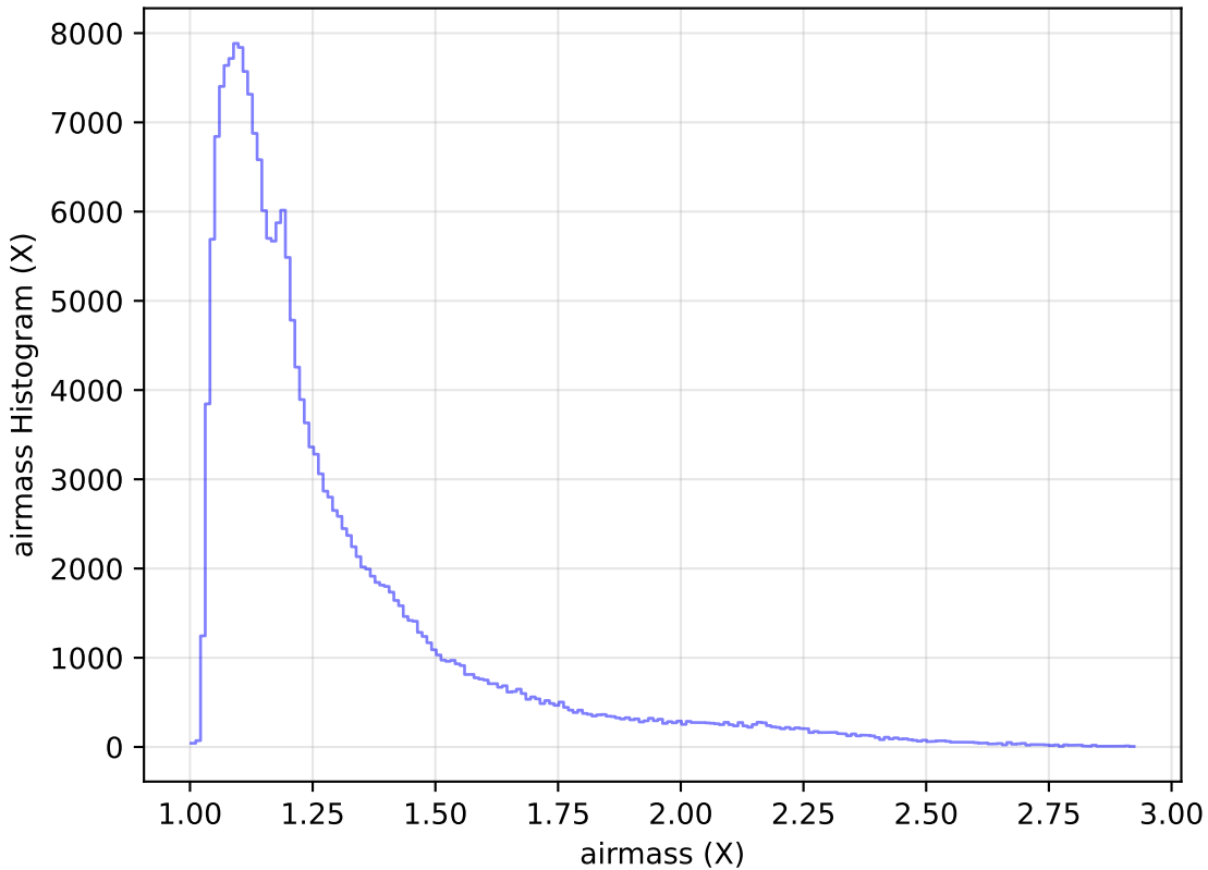
weather_cloudso16v3.4_10yrs Yr 1 all bands: airmass Histogram
