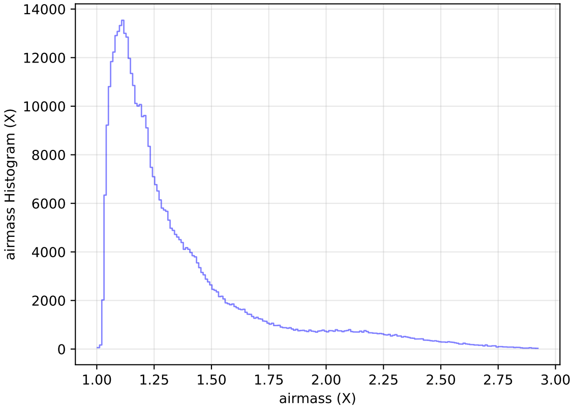
weather_cloudso16v3.4_10yrs WFD z band: airmass Histogram
