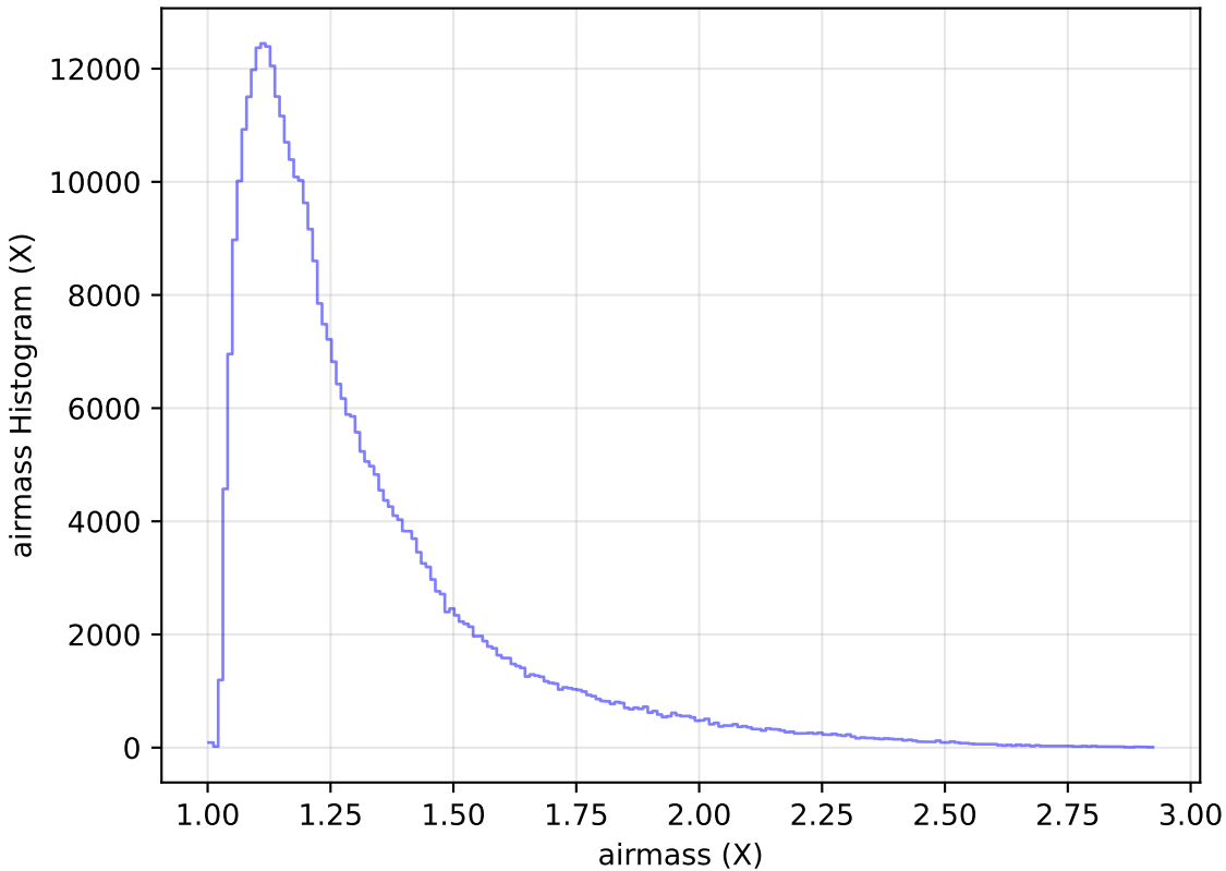
weather_cloudso16v3.4_10yrs WFD y band: airmass Histogram
